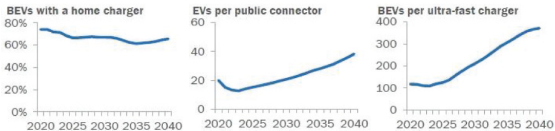
U.S. Passenger EV Charging Infrastructure Demand (a)
